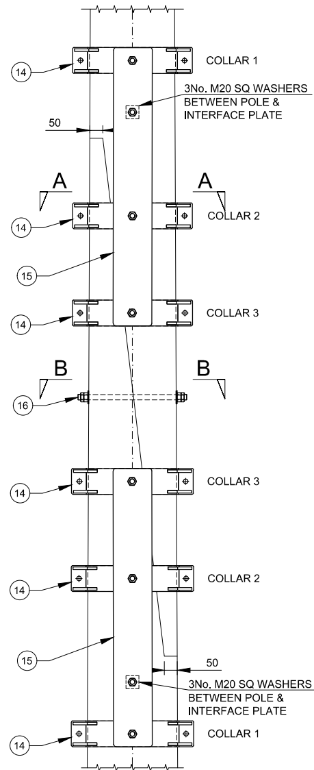
DETAIL I TIMBER POLE SPLICE Scale 1:20
