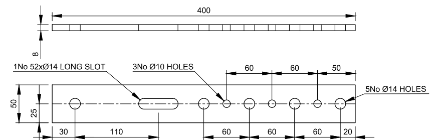
TPA-PD - 8mm THICK Scale 1:5
