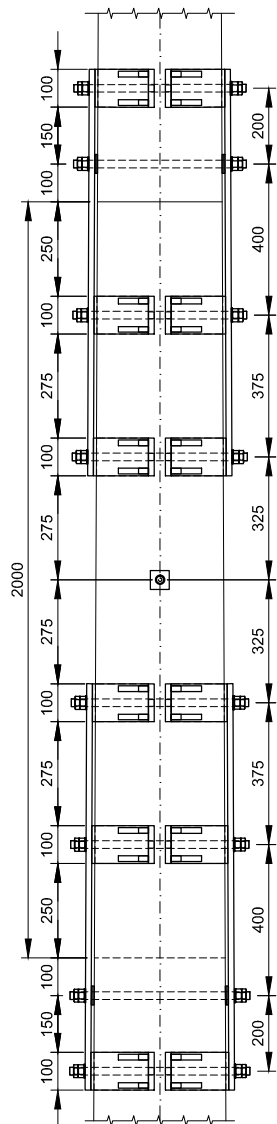
DETAIL I TIMBER POLE SPLICE Scale 1:20
