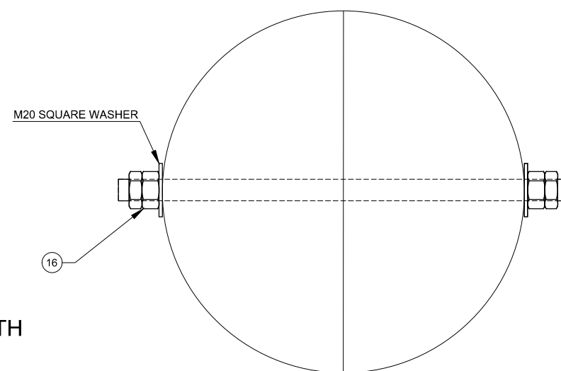
SECTION B-B Scale 1:5
